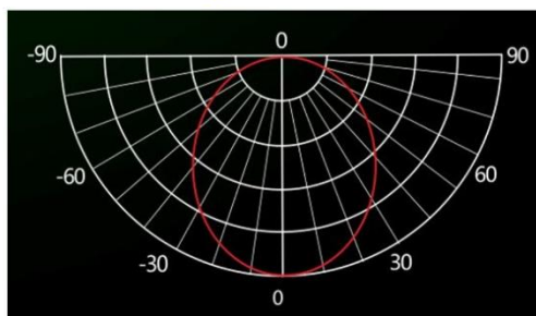
Illuminance Diagram
